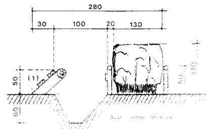
Open-ditch
